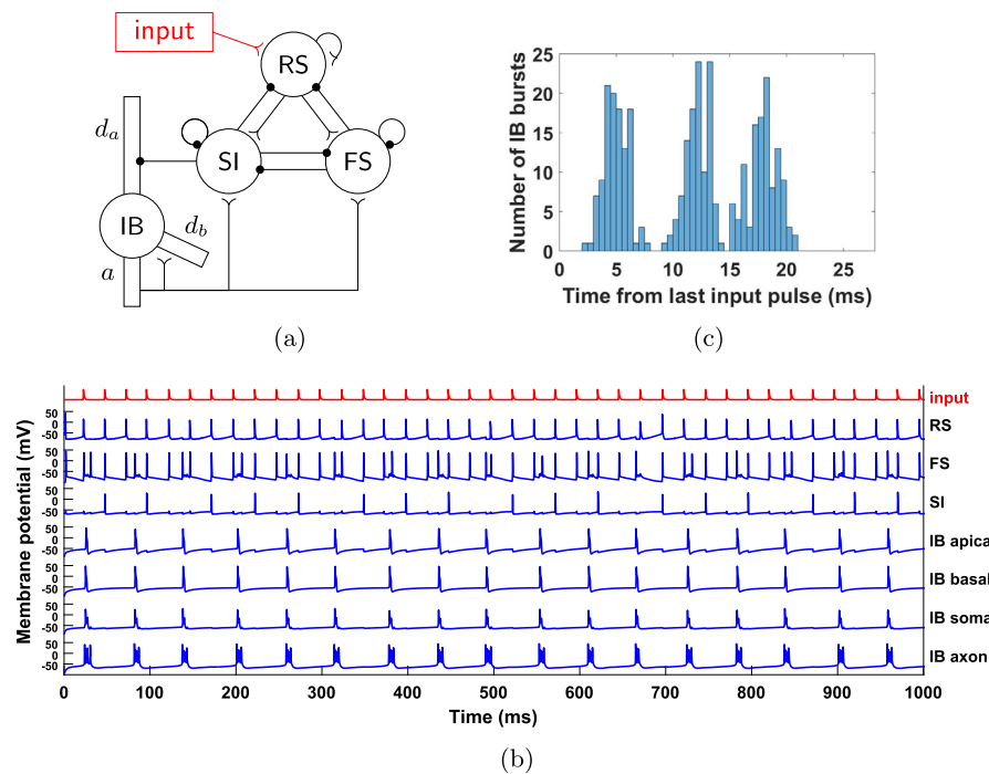
Figure 3 (a) A pulsatile 40 Hz input is given to the RS cell. (b) Same as Fig. 2, but with the RS cell driven by the input (red trace). The SI cell still fires in phase with the RS cell, but its firing rate remains in the beta1 range ( \sim 17 Hz). (c) Histogram of input phase (time from last pulse) when IB cell fires. For each bin, the height of the bar is the number of IB bursts in the simulation having the property that the time elapsed from the last input pulse to the first spike of the burst falls in that bin. The IB cell tends to fire more in certain phases of the external input, showing that the latter is having an effect on the former. Here and in all statistical analysis below, transients are ignored (see Appendix D.2)
