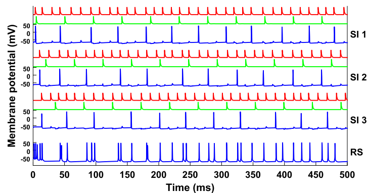
Figure 24 A simulation of the network in Fig. 23(a). Input-2 is 22 Hz and input-1 has average frequency 70 Hz with 10% variability in the interpulse intervals (see Appendix D.1). Above the membrane potential of each of the SI cells, the two inputs that it receives are shown (red for input-1, green for input-2). Each of the SI cells behaves as in the network of Fig. 9. The RS cell fires in response to each of the three SI cells and only to them (with the exception of the transient period). The network as a whole implements the time-division multiplexing mechanism described in Fig. 22
