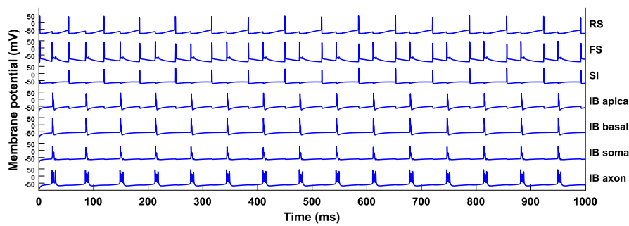
Figure 2 Simulation of the network shown in Fig. 1. Each of the seven blue traces shows the membrane potential of one cell/compartment. All cells fire periodically, with the RS, SI, and IB cells having a frequency of about 15 Hz, and the SI and RS cells being in phase with each other. Parameter values used for all simulations are given in Appendix D.1
