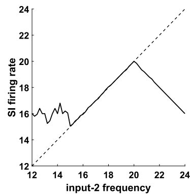
Figure 6 Firing rate of the SI cell as a function of the input-2 frequency, for the network of Fig. 5. For a range of frequencies, the firing rate of the SI cell is equal to the input-2 frequency. Dashed line: diagonal
